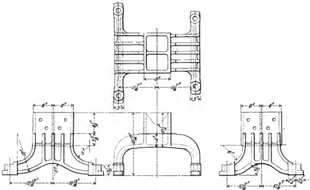
Figs. 3425-3428. Truck Bolster.
